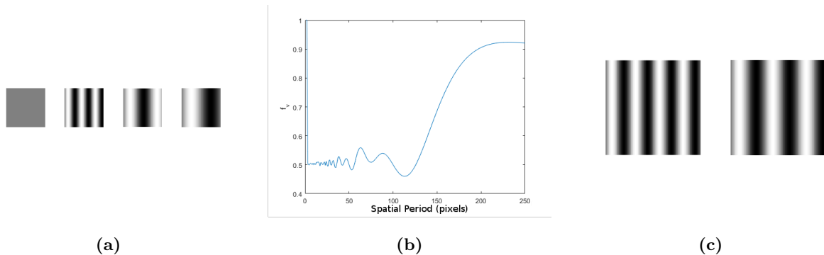
Figure 4: Left: Sinusoidal gratings used as stimulus. The spatial period T_s increases from T_s = 1 pixel (leftmost) to T_s = 100 pixels (rightmost). Center: Uniformity feature f_v of static sinusoidal gratings with respect to gratings' spatial period. Right: The leftmost grating fits exactly in the RF area. Four full periods cover the RF area. For the rightmost spatial grating, approximately 3.5 periods cover the RF area
