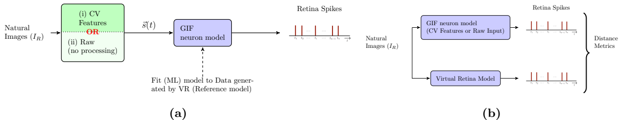
Figure 3: Left: Training Pipeline. (i) The images are processed to extract features (Section 2) . These features are used as input to a GIF model (Section 3.2) which produces the retina spiking output. To determine GIF model parameters, we use data fitting methods. (ii) Alternatively, raw images are directly fed to a GIF model Right: Performance evaluation is based on distance metrics between GIF model spiking response and VR spiking response
